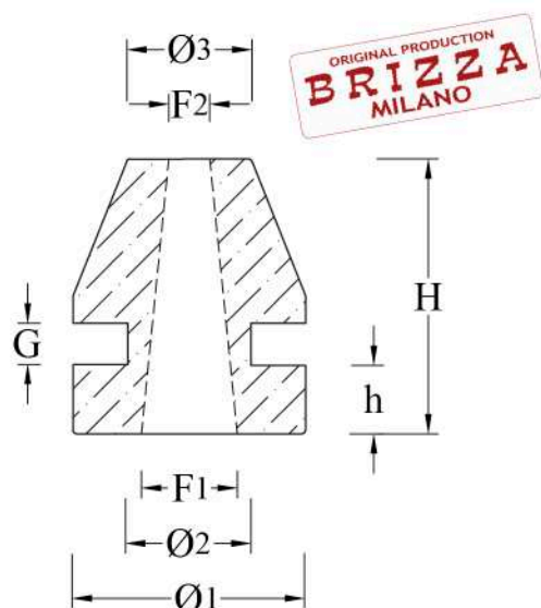
Passacavo a pipetta con foro conico (Art. 3267/100 e simili) Pipette shaped cable gland with conical hole (Art. no. 3267/100 and similar)
