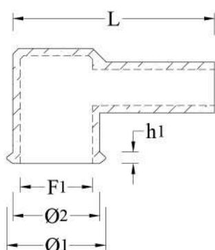
Cappuccio a pipa (Art. 0183/1 e simili) Pipe shaped cover (Art. no. 0183/1 and similar)
