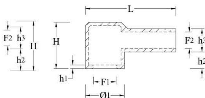
Cappuccio a pipa (Art. 0127/1 e simili) Pipe shaped cover (Art. no. 0127/1 and similar)
