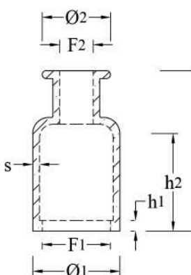
Cappuccio a bottiglia (Art. 3604/30 e simili) Bottle shaped cover (Art. no. 3604/30 and similar)
