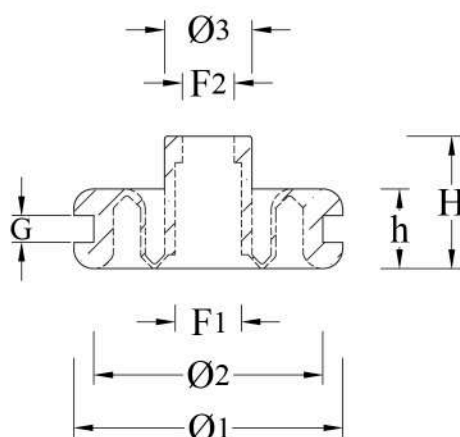
Passacavo a pipetta (Art. 3829/25 - 4044/25 e simili) Pipette shaped cable gland (Art. 3829/25 - 4044/25 and similar)
