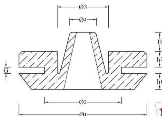
Passacavo a pipetta in Tpe, Pvc e Tpu (Art. 171/10 e simili) Pipette shaped cable gland in TPE, PVC e TPU (Art. no. 171/10 and similar)
